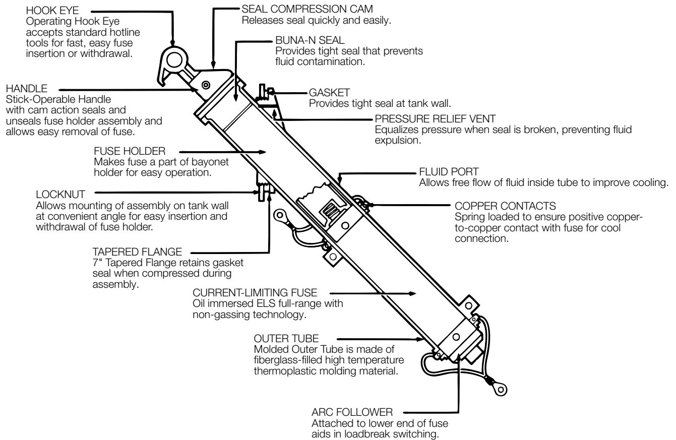
Figure 2. Cutaway shows feature detail with current-limiting fuse mounted.
