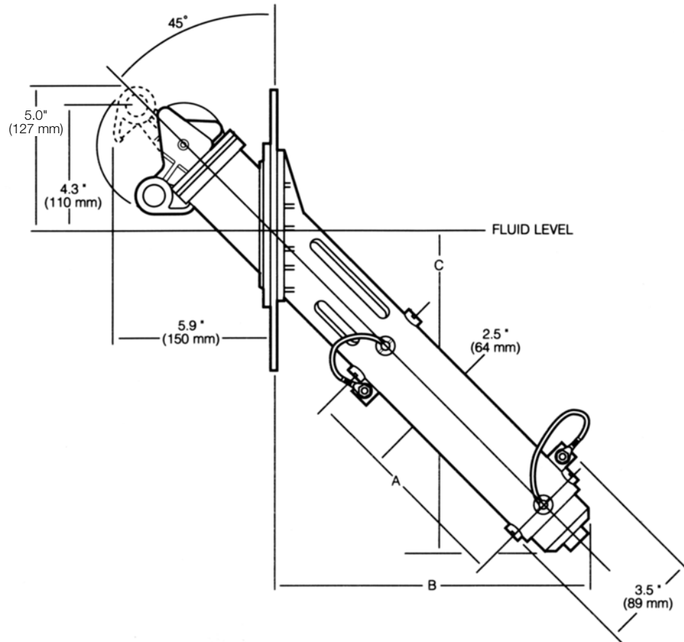
FIGURE 3 Line drawing shows application fluid level and dimensional information.
